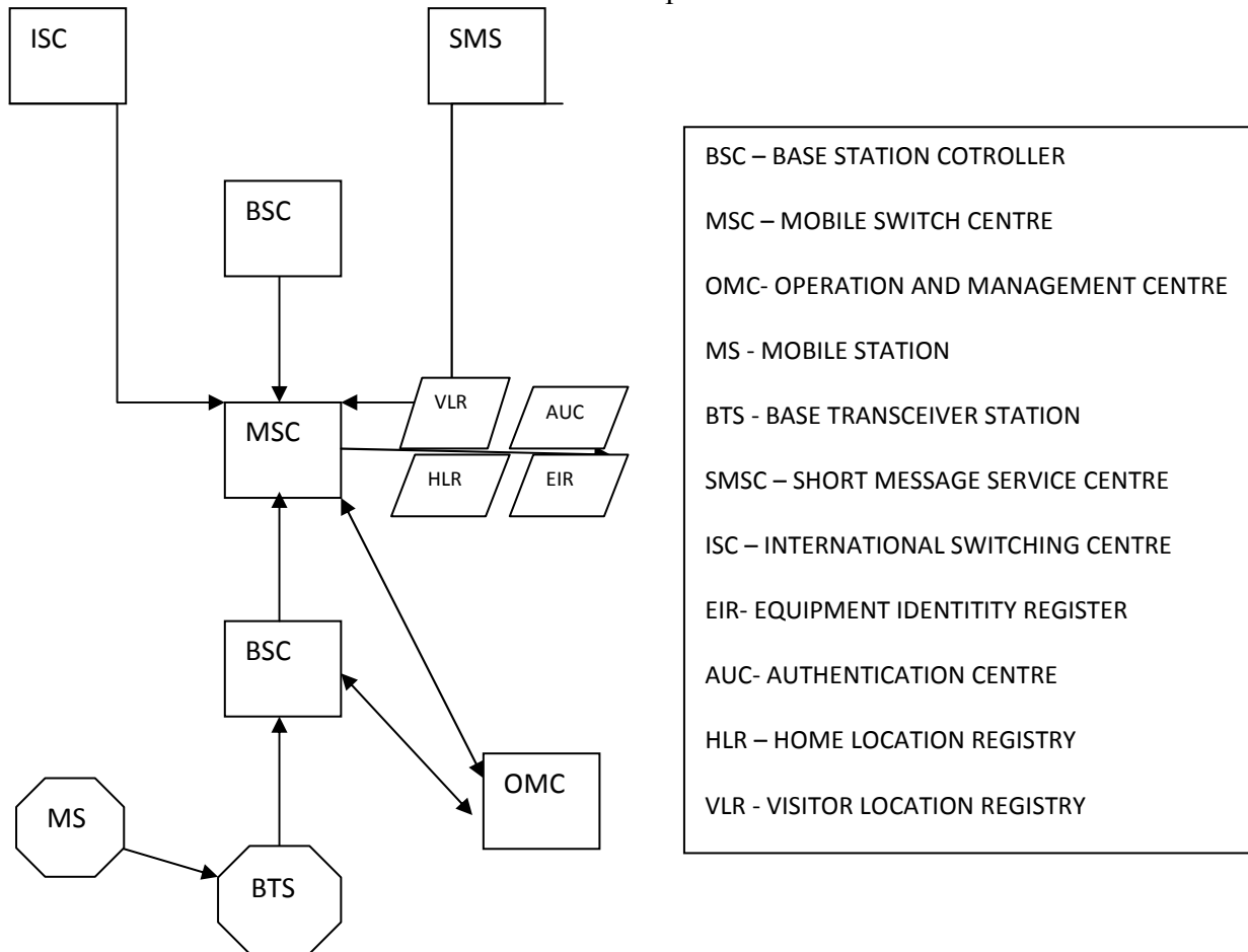
Figure 1. GSM Architecture
